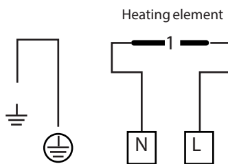
CS20~CS30 Circuit diagram
