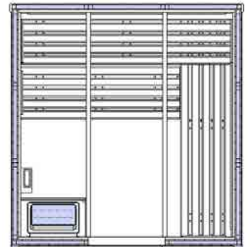
D3030 3-5 bathers 1860 x 1960 x 1950mm
